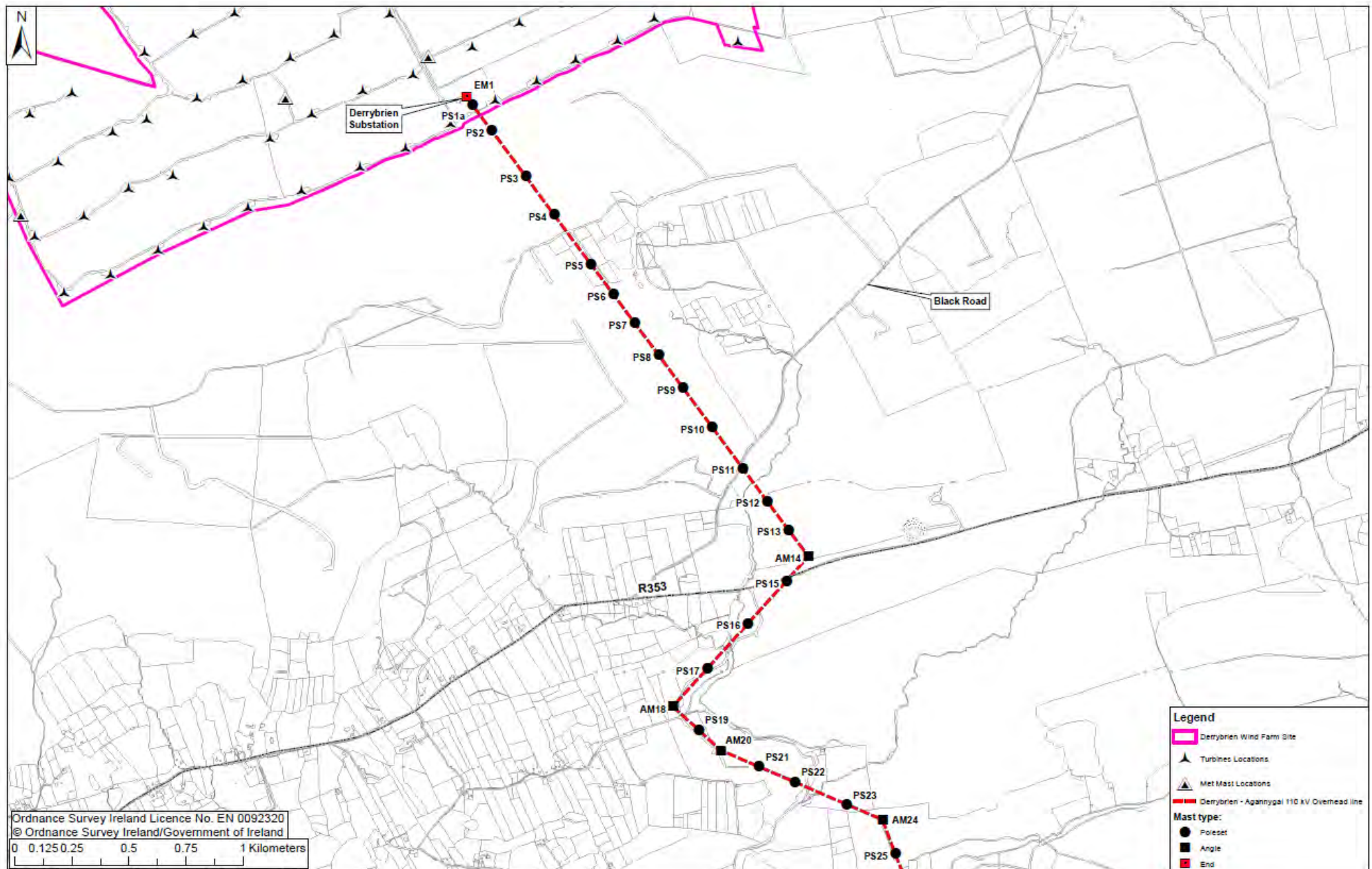
Figure 3-2 Derrybrien - Agannygal 110kV Overhead Line Route (Sheet 1 of 2)
