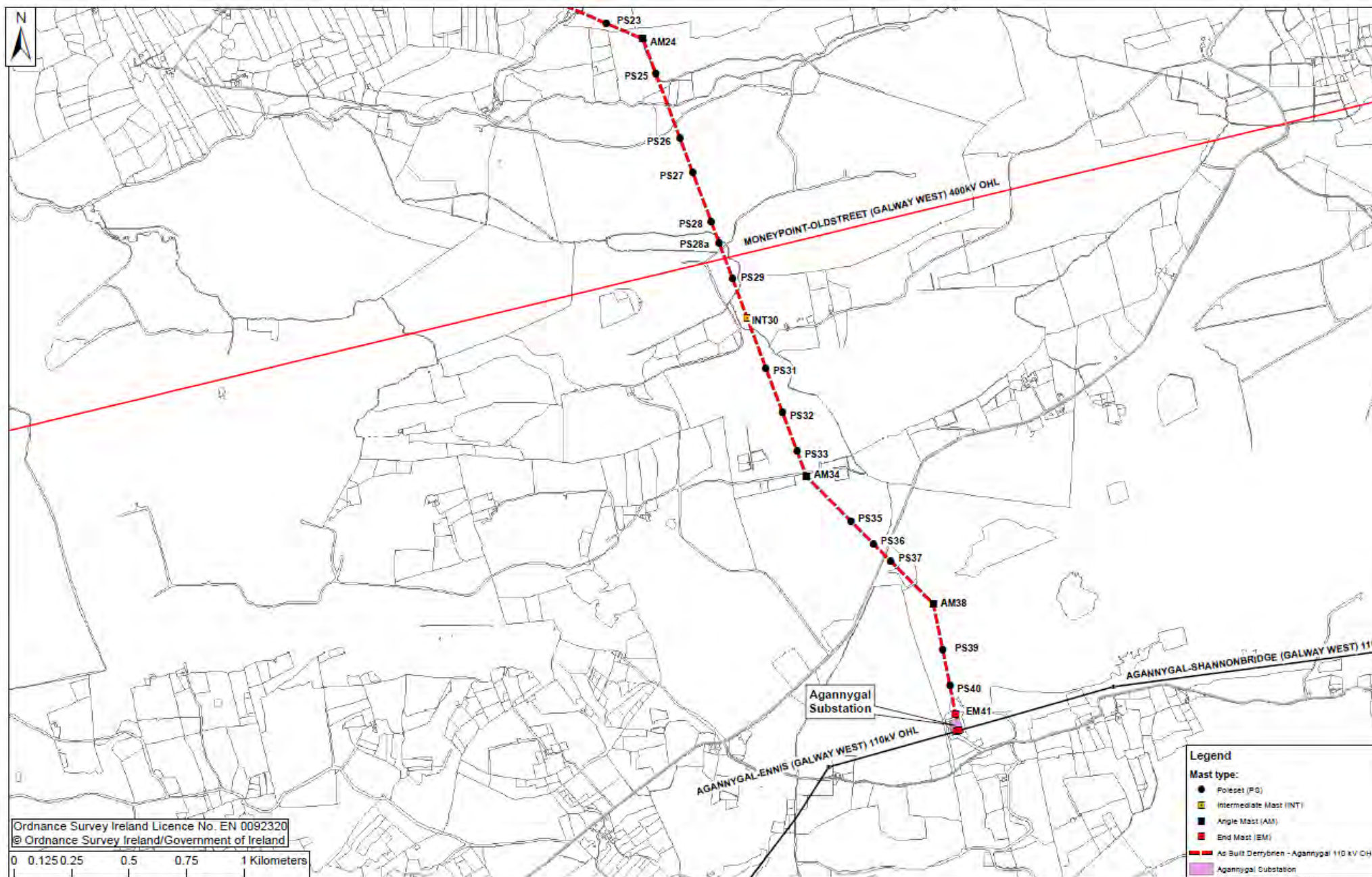
Figure 3-3 Derrybrien - Agannygal 110kV Overhead Line Route (Sheet 2 of 2)
